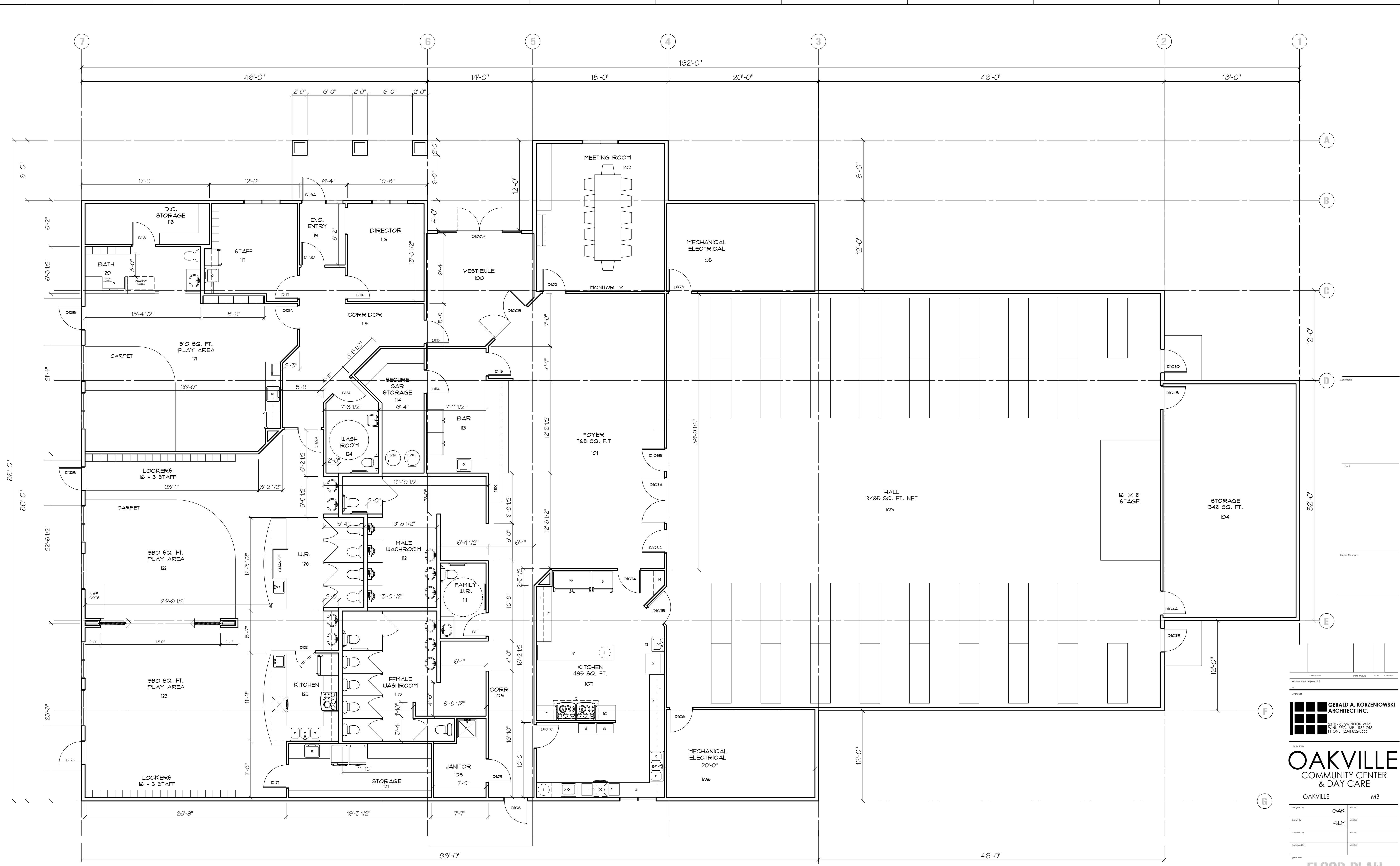
FLOOR PLAN - COMMUNITY CENTER / DAYCARE GROSS BUILDING AREA = 11,018 SQ. FT. (1029.55m 2 )
